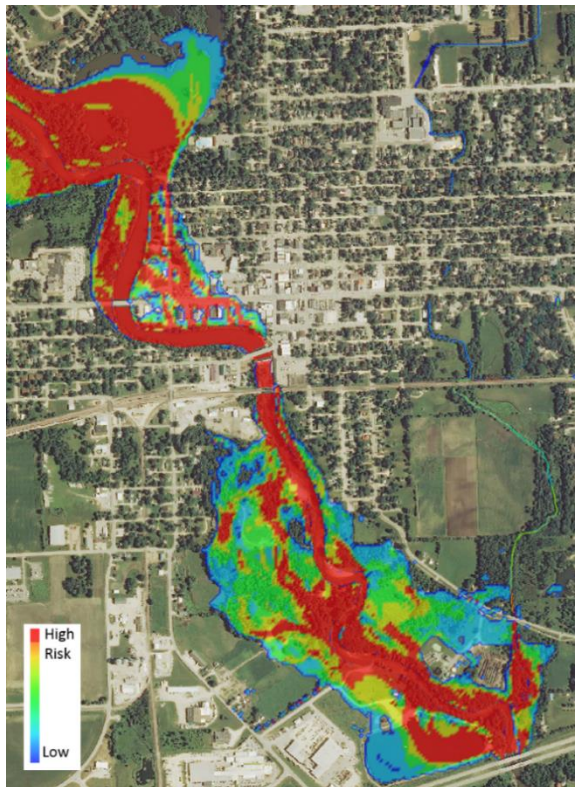
Figure 46. XP-C2 IFC max property safety risk for the July 2010 event compared to photos
