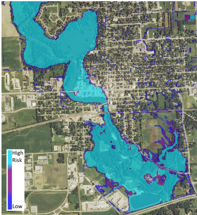
Figure 45. XP-C2 IFC max road safety risk for the July 2010 event compared to photos
