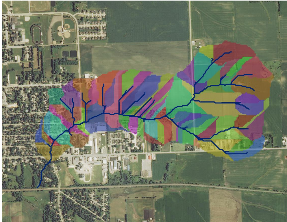
Figure 9. The land surface representation as hillslopes and links by the HLM
