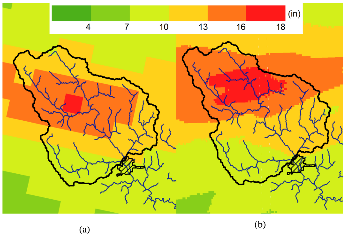
Figure 12. A comparison of the accumulated precipitation over the upper Maquoketa watershed for the July 2010 flood event with (a) StageIV and (b) IFC radar rainfall estimates
